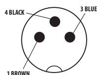
3 PIN MALE
