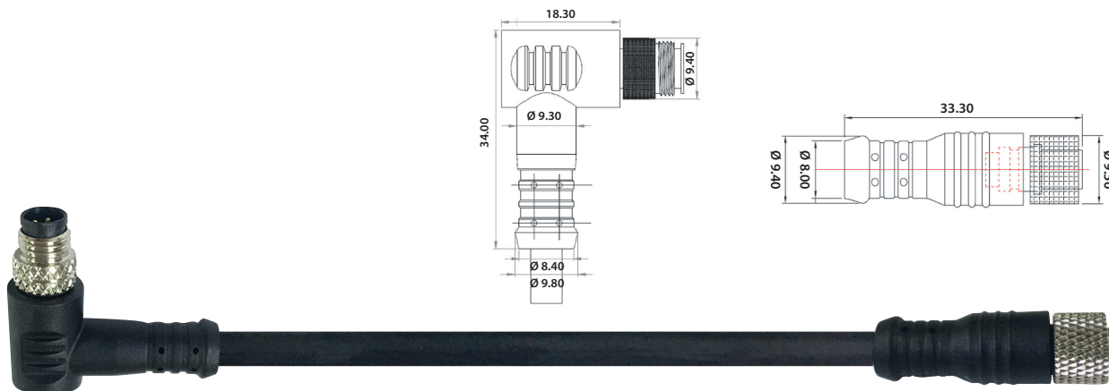
3 PIN MALE
