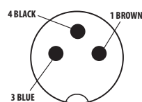
3 PIN FEMALE
