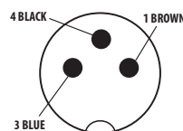
3 PIN FEMALE
