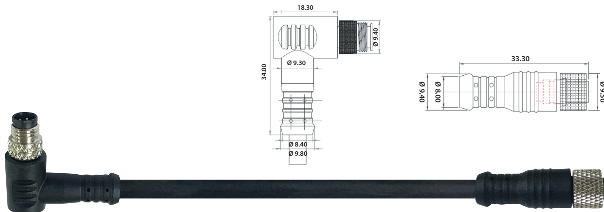
3 PIN MALE
